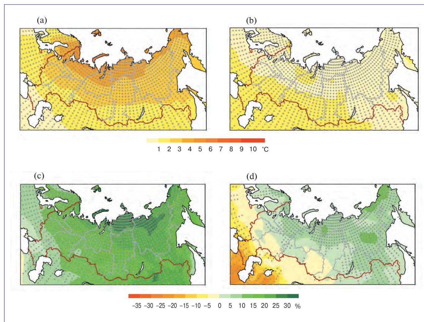
Fig. GS7. Changes in surface air temperature (a, b) and total (solid and liquid) precipitation (c, d) in Russia and adjoining regions for winter (a, c) and for summer (b, d) during the period 2041–2060, as compared to the period 1980–1999. Assessment was obtained from the ensemble of 16 CMIP3 AOGCMs using scenario A2. Temperature is given in degrees Celsius and precipitation in percent relative to its value in the corresponding season for the period 1980–1999. In the upper panels (a, b) dots imply that mean temperature changes exceed the standard deviation of the inter-model scatter (signal is larger than noise), and in the low panels (c, d) they denote the areas where two thirds of the models show changes of the same sign (AR, vol. 1, Figs. 7.7, 7.14).
