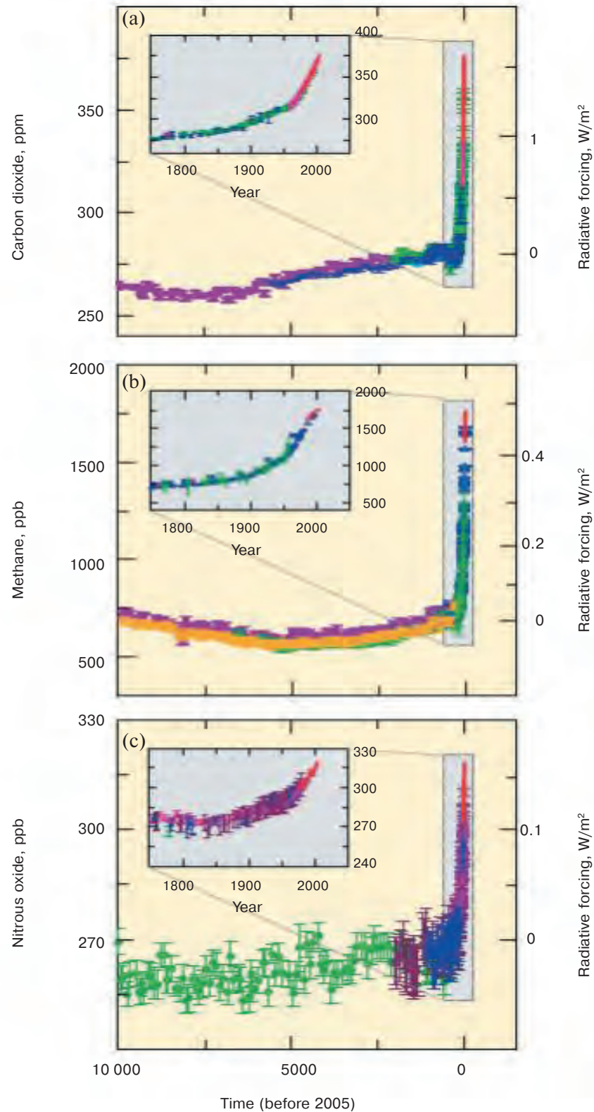
Fig. GS3. Time dependence of the concentration of carbon dioxide (a), methane (b) and nitrous oxide (c) in the atmosphere over the past 10 000 years (large panels) and since 1750 (inset panels). Measurements are shown from ice cores (symbols with different colors from various studies) and atmospheric samples (red lines). The corresponding radiative forcings are shown on the right hand axes of the large panels (AR, vol. I, Fig. 4.1).
